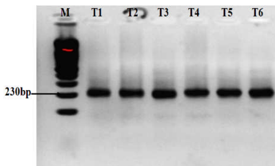
Figure 3: DGGE-PCR amplified from 16S rDNA at V3 region (200 ~ 230 bp)
