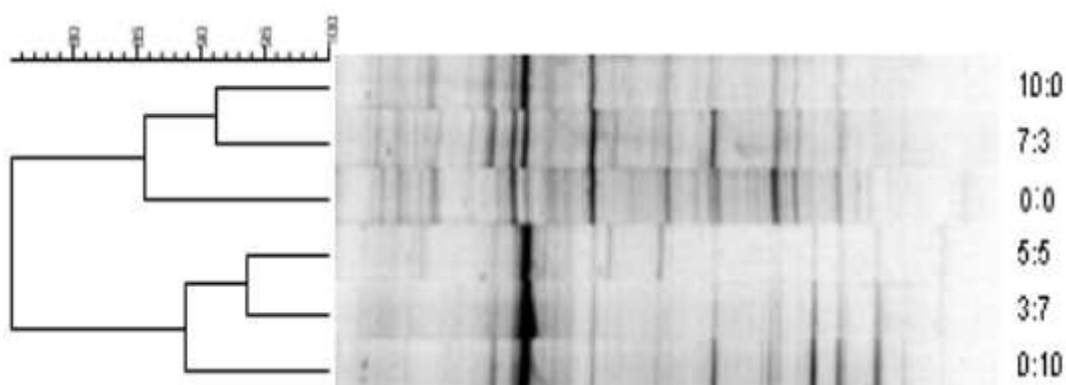
Figure 5: UPGMA cluster analysis of DGGE band pattern of amplified 16S rDNA V3 region from rumen in vitro fermentation.
