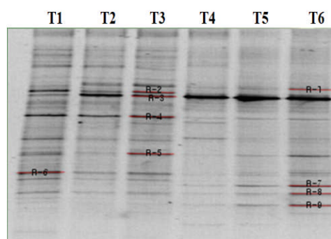
Figure 4: Negative image of DGGE gel bands which were divided from amplified 16S rDNA at V3 region
